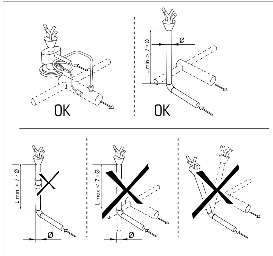
13 - Montage Expansionsventil
