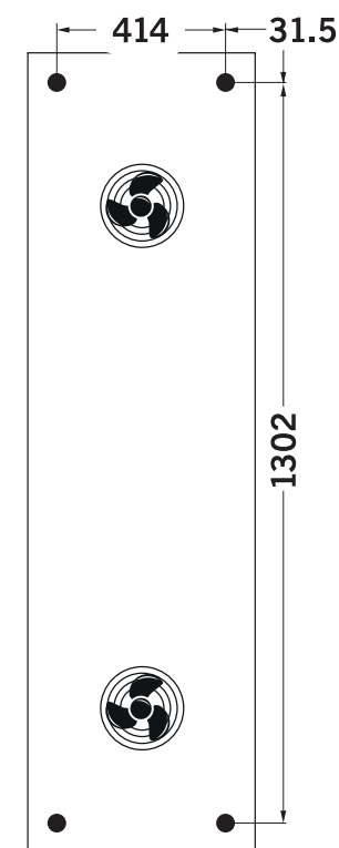
GAMC 020.1/2**/DY***
