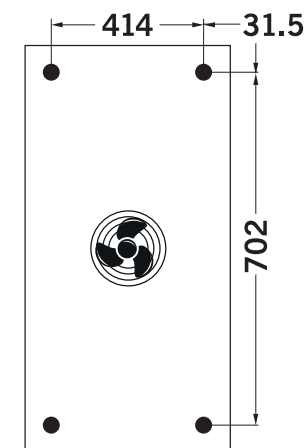
GAMC 020.1/2**/DY***
