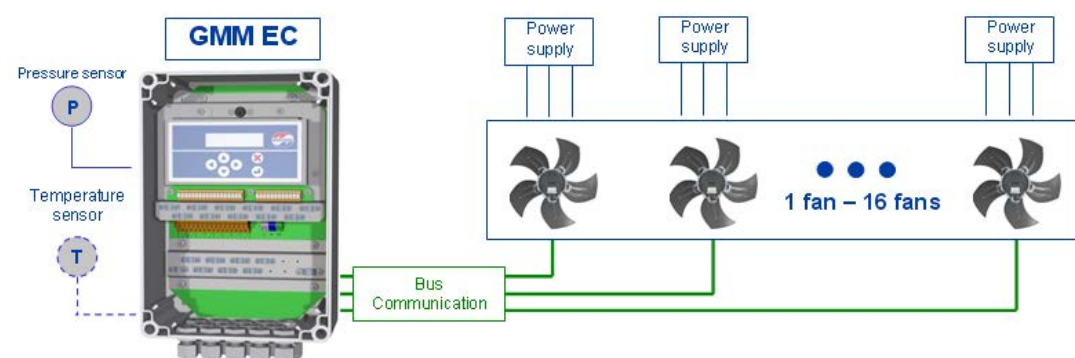
Figure 3: System Configuration with EC fans + GMM.
