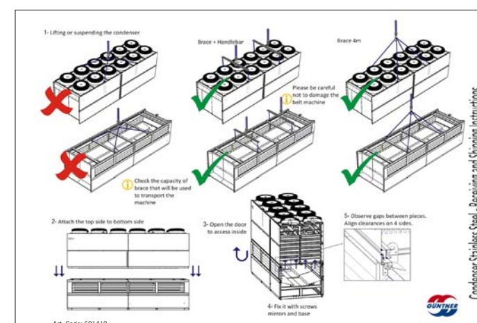
Figure 5: Instructions for receiving, handling and assembly of upper and lower modules.
